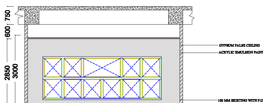
ELEVATION D
