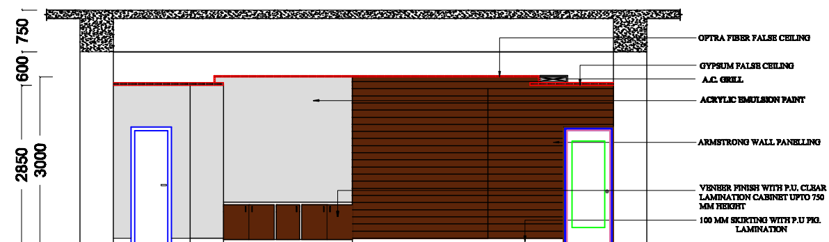
ELEVATION AT A
