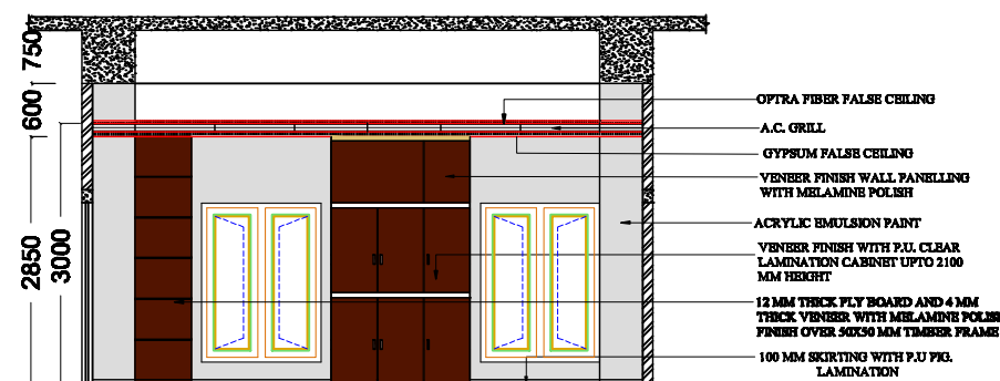
ELEVATION AT B
