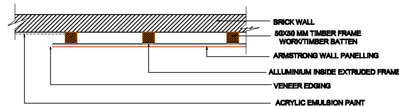
DETAILS AT 'X'
