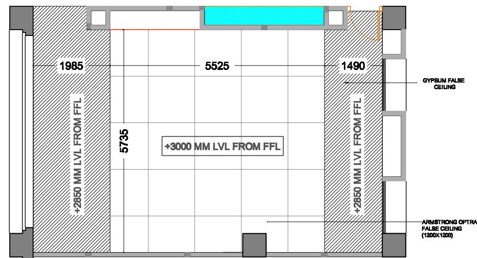
REFLECTED CEILING PLAN LAYOUT
