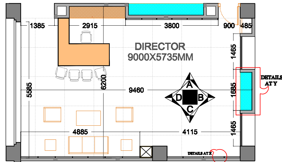
FURNITURE LAYOUT OF THE DIRECTOR'S CABIN-3
